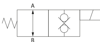
2. Poppet 2-way double lock normally open
